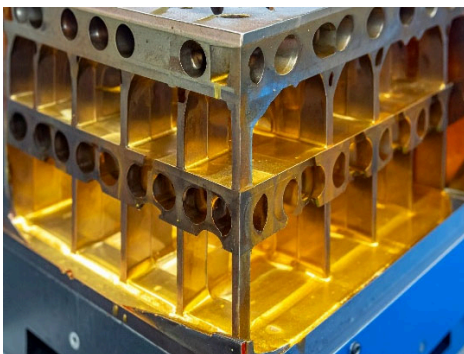
Illustration of a corner of conventionally made breeding blanket structure. Illustration by S. Wikman.
